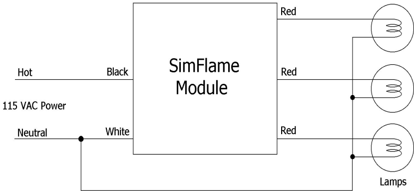
Wiring Diagram
