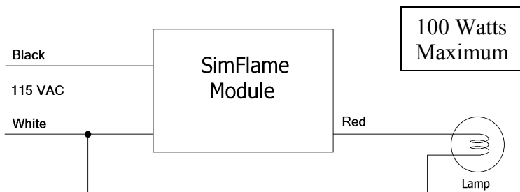
Wiring Diagram
